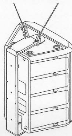
FIGURE 7 — Suspending the Sx200a Using the Mb200 Installation Kit
